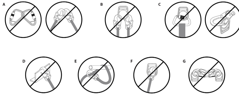
Figure 3 - Non-Compatible Connections
